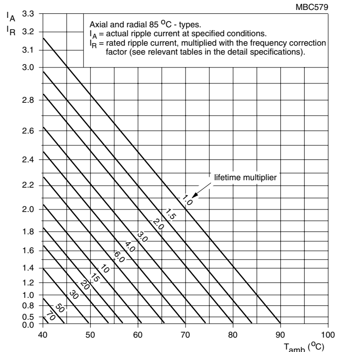
Fig.15 Typical example of a life-time nomogram: useful life as a function of ambient temperature and ripple current load.
