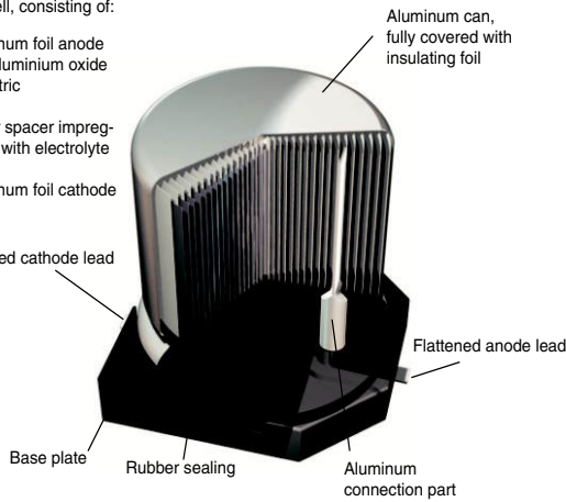
Fig.4 Surface Mount Device (vertical style).
