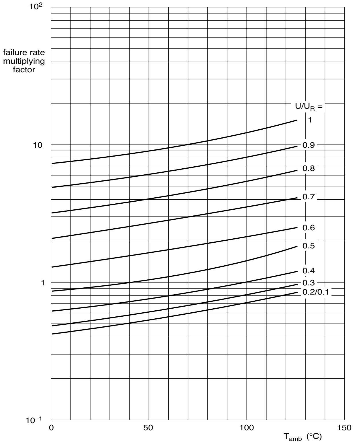
Fig.19 Conversion factors for failure rate ( \lambda ) as a function of ambient temperature ( T_{amb} ) and voltage ratio ( U/U_R ) for solid aluminum capacitors.
