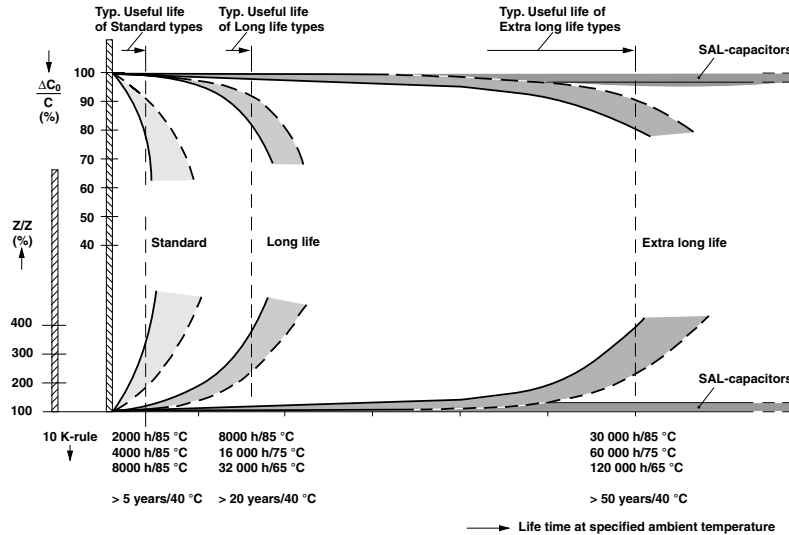
Fig.14 Principal trend of electrical parameters during useful life of different aluminum capacitors
