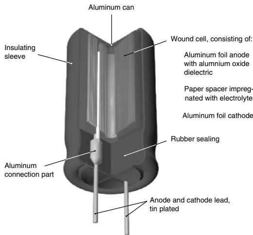
Fig.5 Radial Aluminum.
