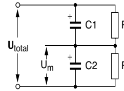
Fig.20 Balancing resistors for two aluminum capacitors in series.
