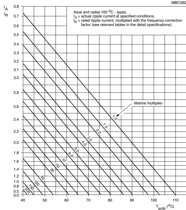
Axial and radial 105 °C types.
