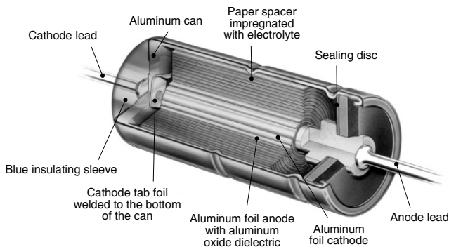
Fig.6 Axial Aluminum.
