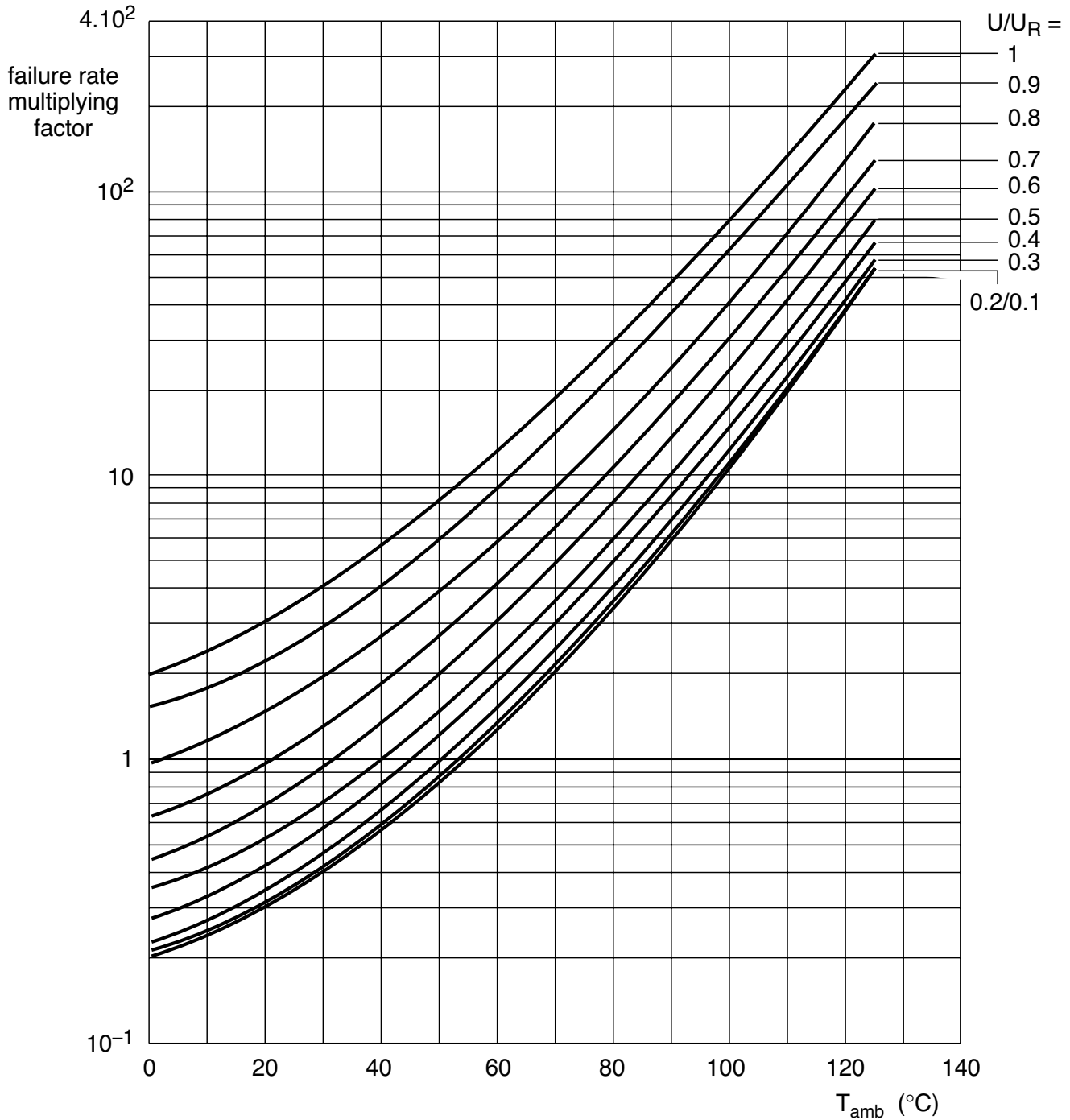
Fig.18 Conversion factors for failure rate ( \lambda ) as a function of ambient temperature ( T_{amb} ) and voltage ratio ( U/U_R ) for non-solid aluminum capacitors.
