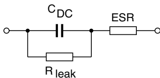
Fig.11 DC equivalent circuit of an aluminum capacitor.
