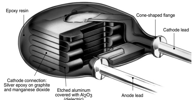
Fig.8 Solid Aluminum (SAL), radial.
