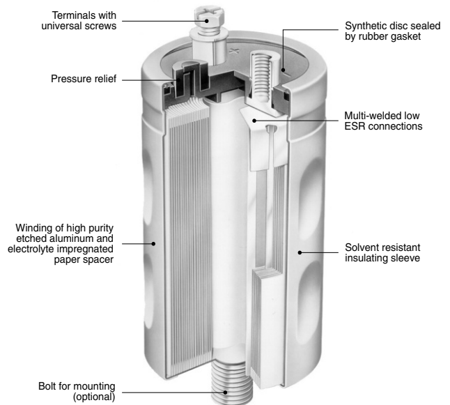
Fig.9 Large Aluminum, screw terminal.
